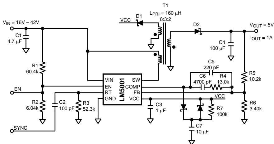
Figure 18. Non-Isolated Flyback
