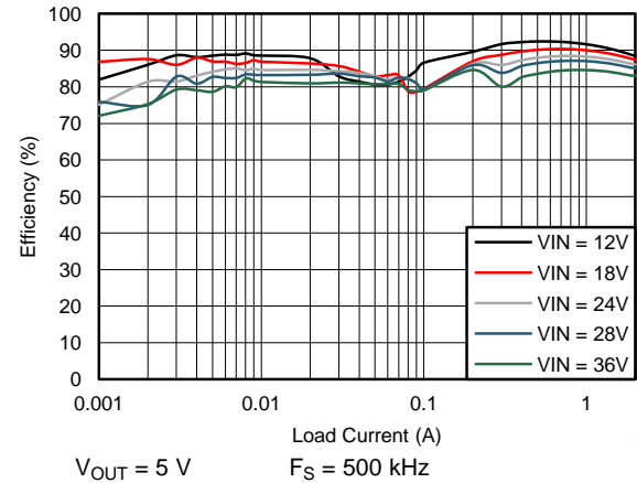
Figure 54. Efficiency
