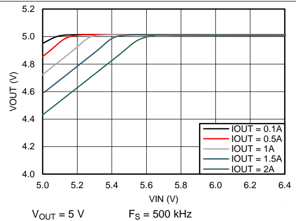
Figure 56. Dropout Curve
