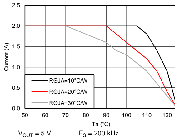
Figure 64. Derating Curve
