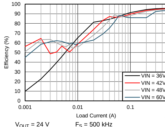
Figure 78. Efficiency
