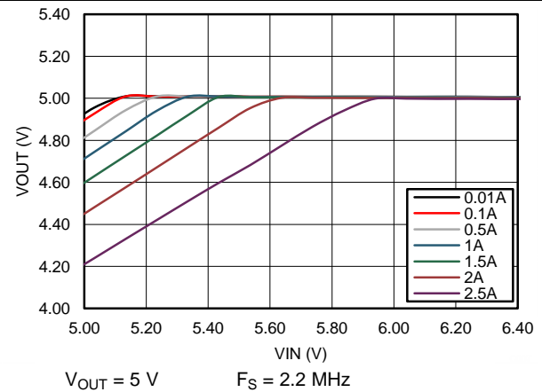
Figure 88. Drop-out Curve
