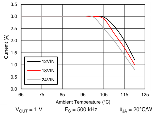
Figure 54. Derating Curve
