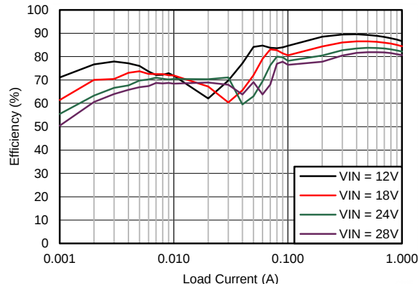
Figure 72. Efficiency
