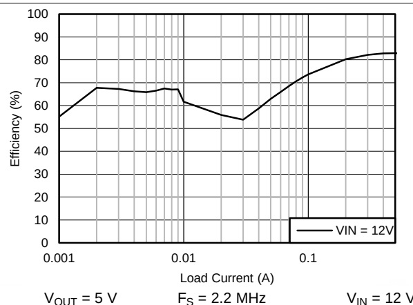
Figure 78. Efficiency
