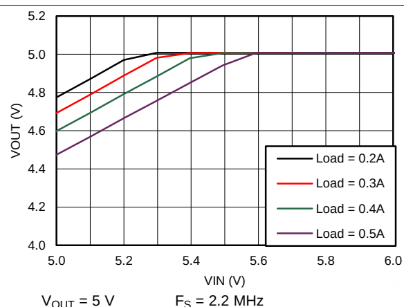
Figure 80. Dropout Curve
