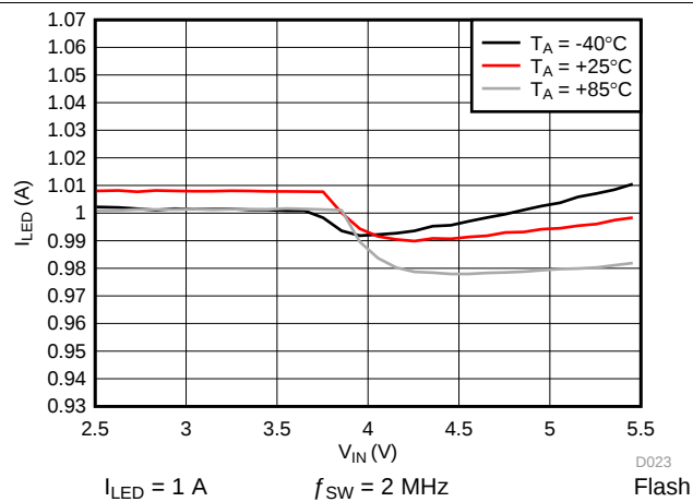
Figure 10. LED1/2 Current vs Input Voltage
