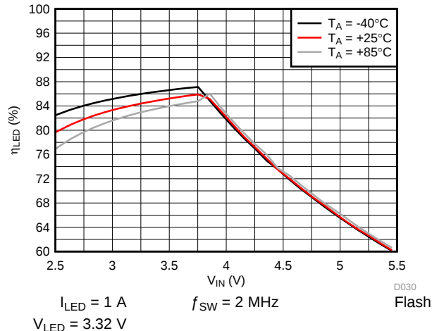
Figure 41. LED Efficiency vs Input Voltage
