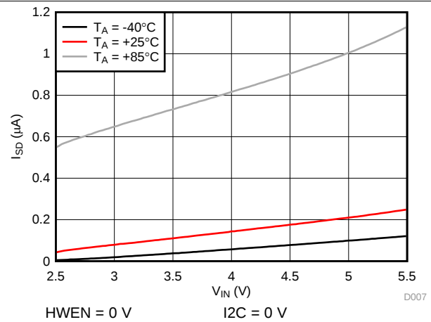
Figure 17. Shutdown Current vs Input Voltage
