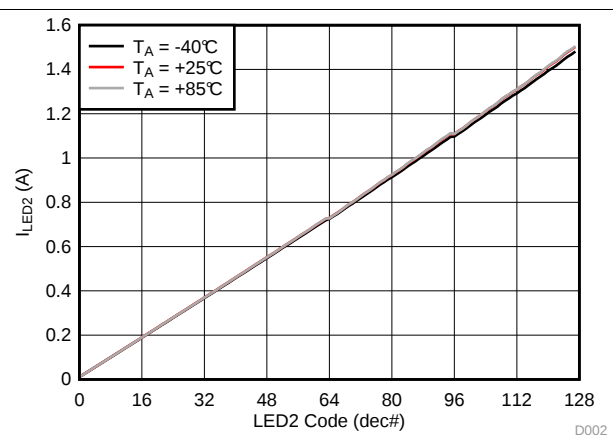
Figure 3. LED2 Flash Current vs Brightness Code
