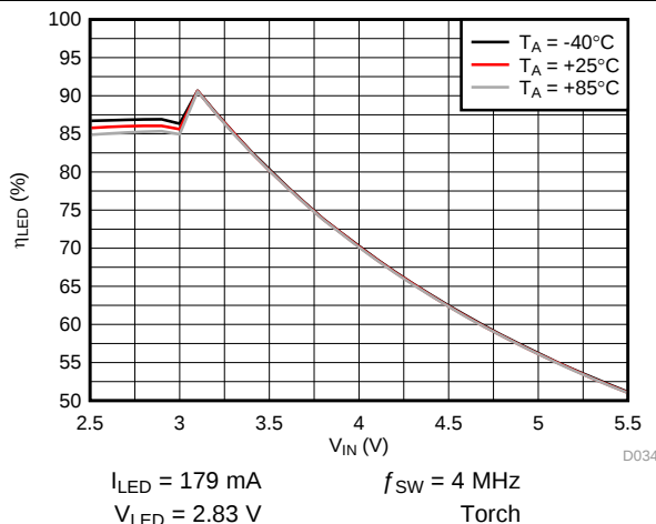
Figure 45. LED Efficiency vs Input Voltage
