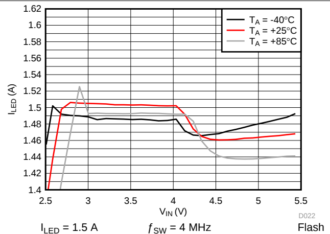
Figure 11. LED1/2 Current vs Input Voltage
