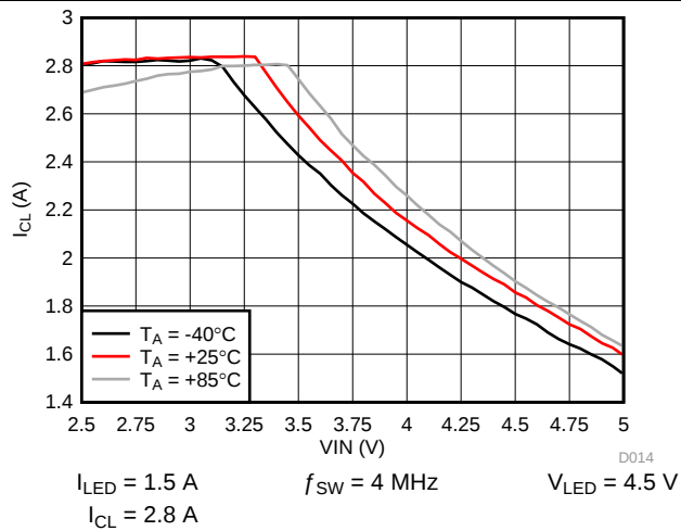
Figure 24. Inductor Current Limit vs Input Voltage
