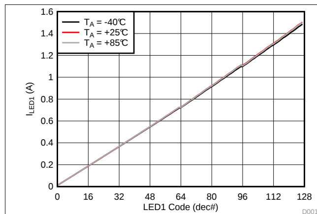
Figure 2. LED1 Flash Current vs Brightness Code
