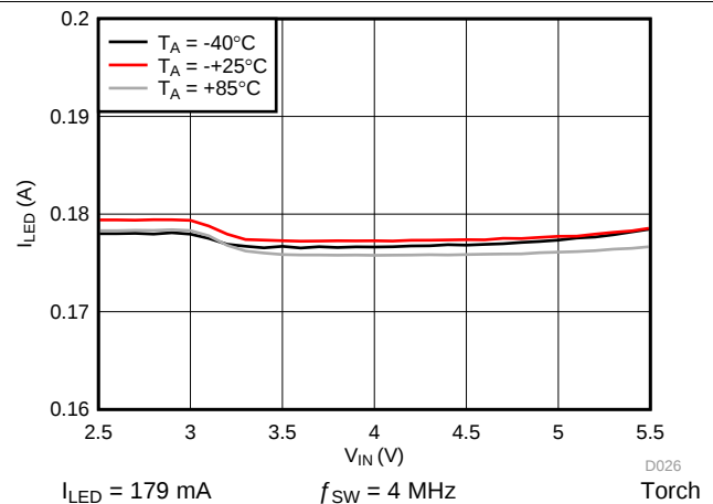
Figure 13. LED1 and LED2 Current vs Input Voltage
