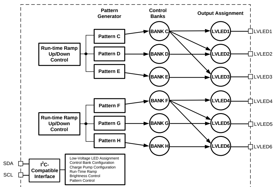
Figure 17. Low-Voltage LED Functional Control Diagram
