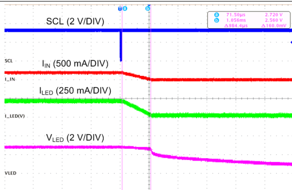
Time (1 ms/DIV) Mode bits (Reg 0x01 bit[1:0]) = 00 (Standby mode)
