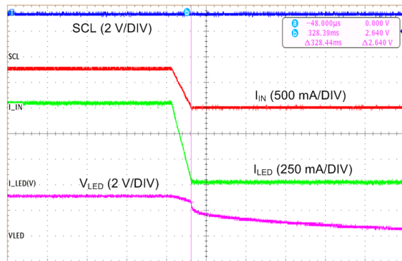
Time (2 ms/DIV) Mode bits (Reg 0x01 bit[1:0]) = 10 (Torch mode)
