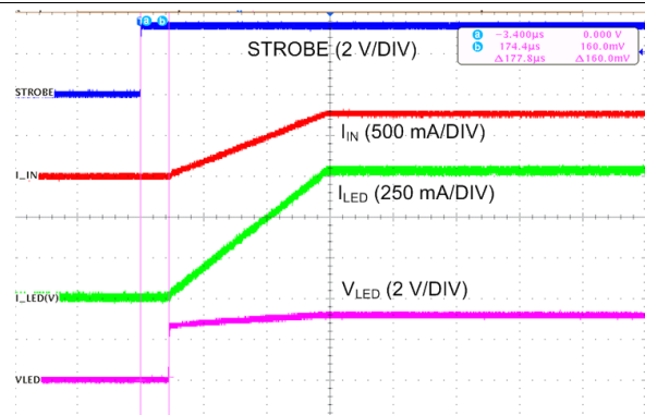
Time (400 \mu\text{s} /DIV) STROBE Enabled (Reg 0x01 bit[2] = 1)
