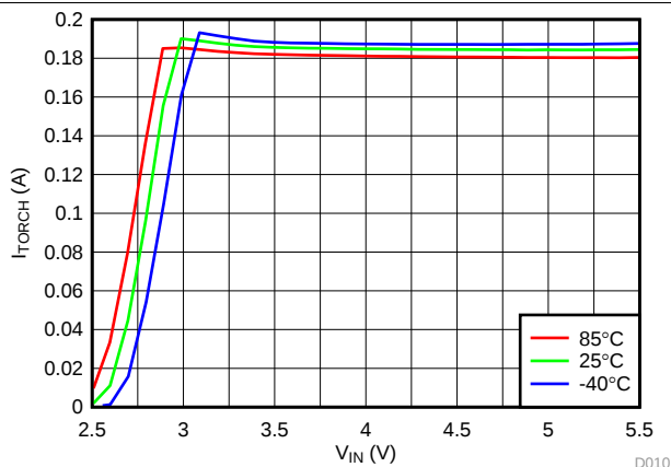
图 9. LED Torch Current vs Input Voltage
