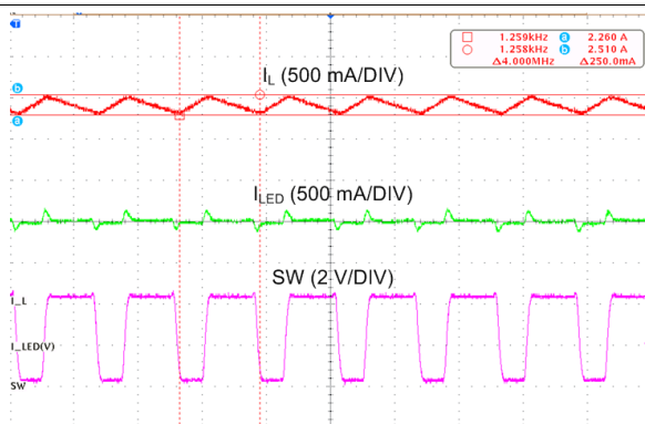
图 77. Pass mode Level Triggered Flash
