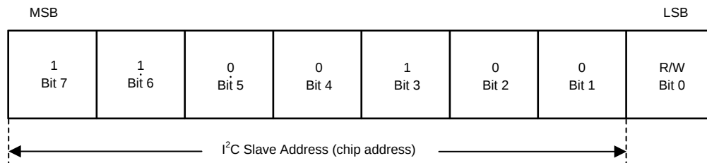
图 36. I 2 C-Compatible Chip Address
