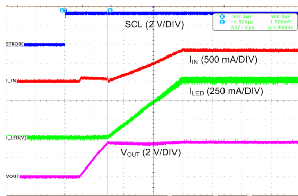
Time (400 \mu\text{s} /DIV) STROBE Enabled (Reg 0x01 bit[2] = 1)
