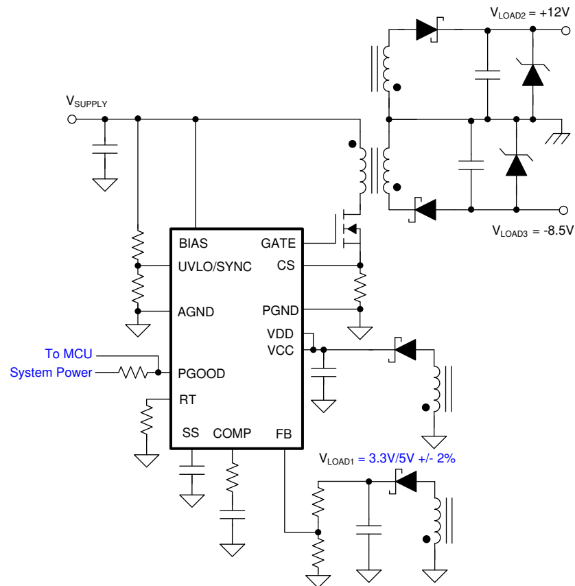
图 9-11. Primary-Side Regulated Multiple-Output Isolated Flyback
