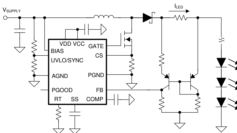
图 9-13. LED Driver with High-Side Current Sensing
