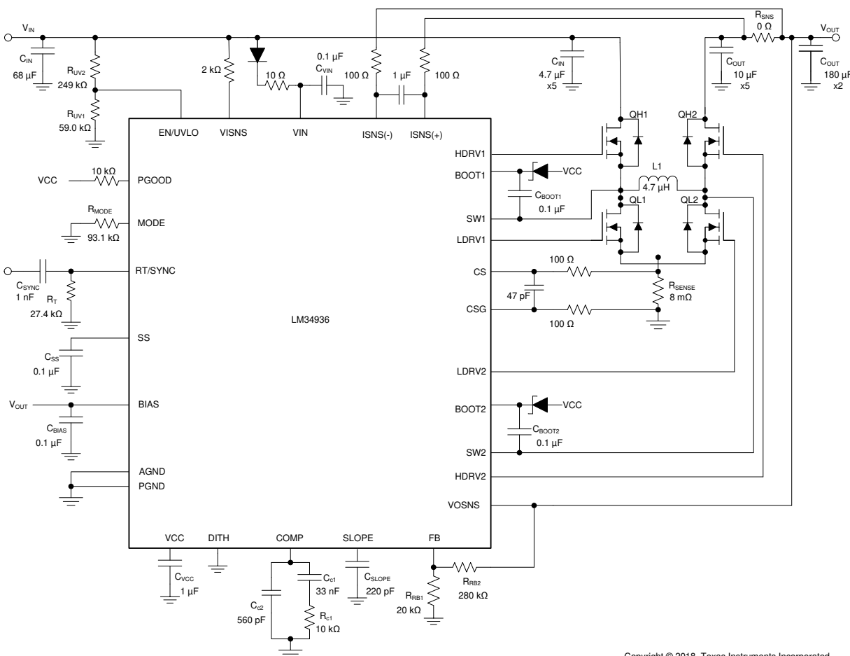
图 8-1. LM34936 Four-Switch Buck Boost Application Schematic
