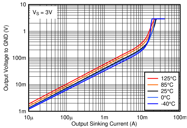
图 2-19. Output Low Voltage vs. Output Sinking Current at 3V
