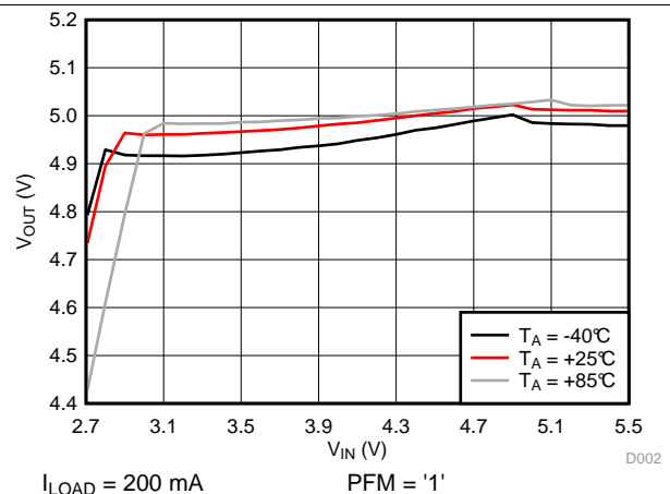
Figure 2. PFM Output Regulation
