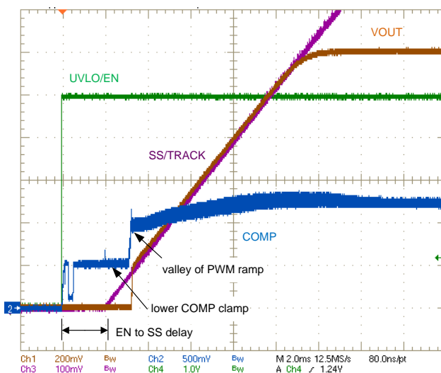
图 35. Typical Monotonic Output Voltage Startup Waveforms, 1.2-V Output
