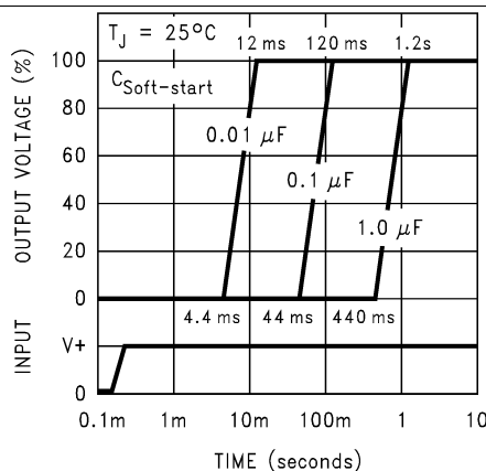
Figure 16. Soft-Start Response
