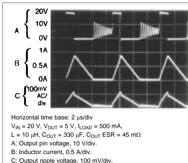
Figure 44. Discontinuous Mode Switching Waveforms
