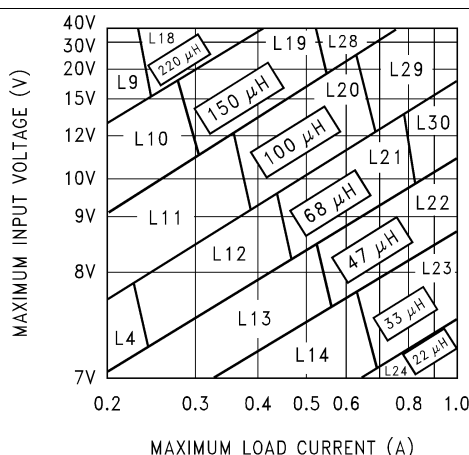
Figure 28. LM2595 5-V
