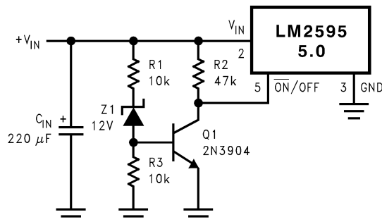
Figure 15. Undervoltage Lockout for Buck Regulator
