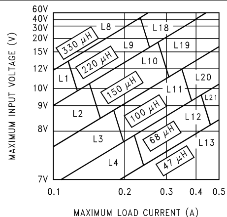
Figure 9-6. LM2594xx 5-V
