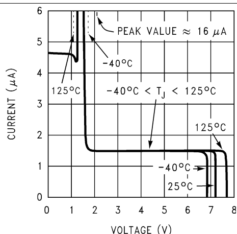
Figure 15. Shutdown/Soft-Start Current
