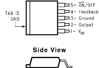
图 5-3. DDPK/TO-263 (S) Package 5-Lead Surface-Mount Package Top View
