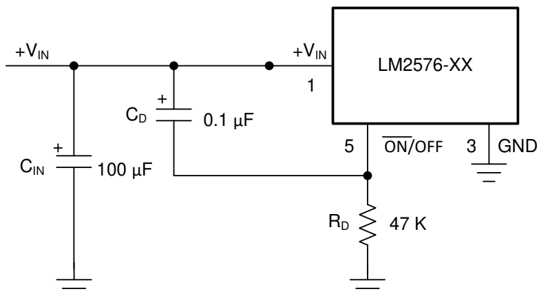
图 7-3. Delayed Start-Up
