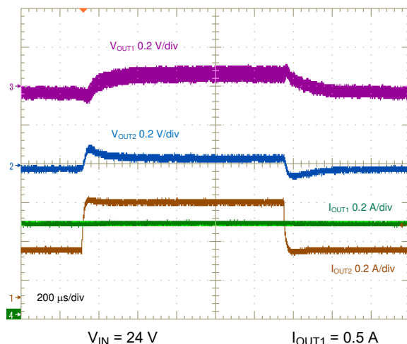
V_{IN} = 24\text{ V} I_{OUT1} = 0.5\text{ A} 图 8-26. Negative Output Load Transient, 0.25 A to 0.5 A
