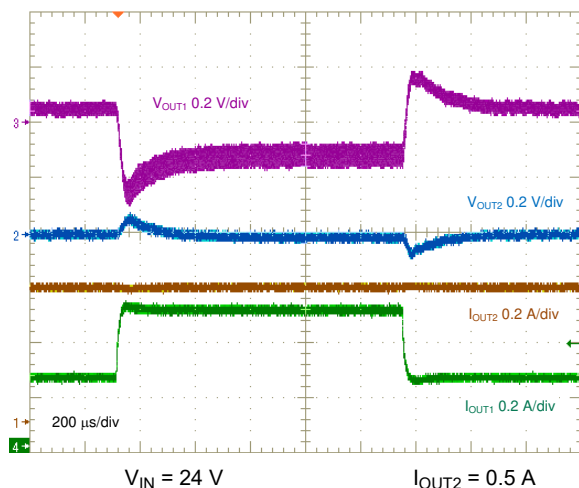
V_{IN} = 24\text{ V} I_{OUT2} = 0.5\text{ A} 图 8-25. Positive Output Load Transient, 0.25 A to 0.5 A
