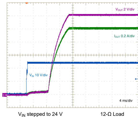
图 8-6. Start-up Characteristic
