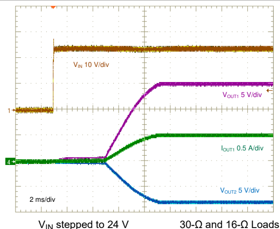
图 8-21. Start-Up Characteristic
