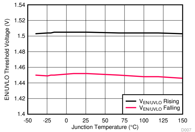
图 6-10. EN/UVLO Threshold Voltages versus Temperature
