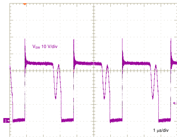
图 8-23. Switch Voltage, Medium Load
