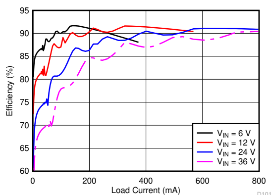
典型效率 ( V_{OUT} = 12V )
