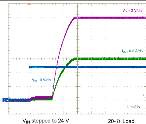
图 8-6. Start-up Characteristic
