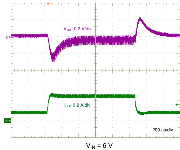
图 8-13. Load Transient, 0.1 A to 0.3 A, 0.1 A/μs
