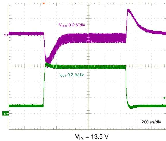
图 8-12. Load Transient, 0.1 A to 0.6 A, 0.1 A/μs
