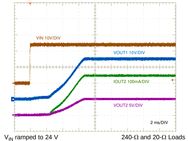
图 47. Start-Up Characteristic
