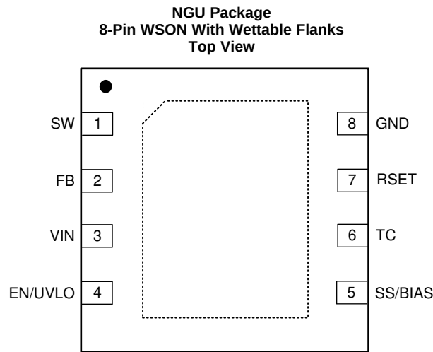
Pin Functions
