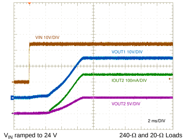
图 47. Start-Up Characteristic
