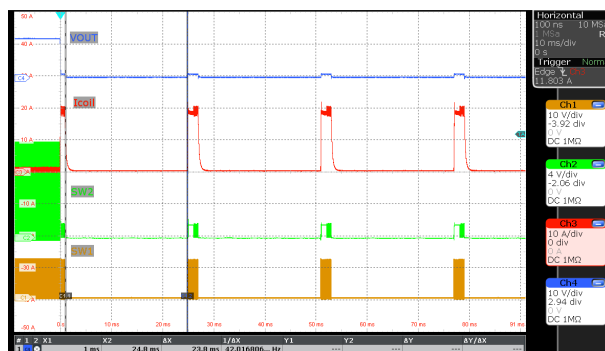
图 10-17. SCP ( V_{(VIN)} = 12V , V_{(VOUT)} = 12V , I_O = 短路, MODE = VCC2 )
