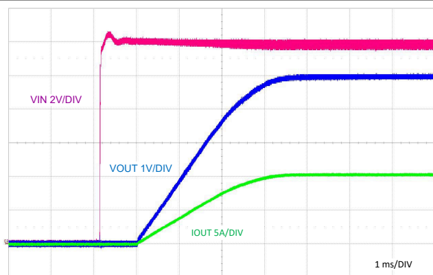
图 9-25. Start-Up Characteristic
