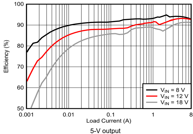
图 9-7. Efficiency vs I_{OUT} , Log Scale
