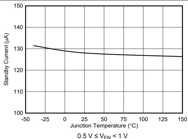
图 7-4. Standby Current vs Temperature
