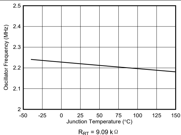
图 7-22. Switching Frequency vs. Temperature
