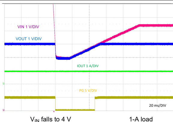
图 9-24. Line Transient Response to V_{IN} = 4 V
