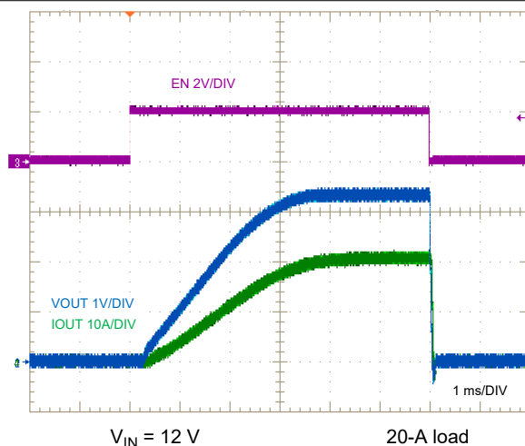
图 9-33. ENABLE ON and OFF Characteristic
