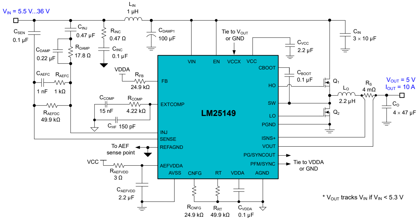
图 9-18. Application Circuit 2 With LM25149 Buck Regulator at 440 kHz
