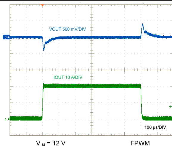
图 9-35. Load Transient, 0 A to 20 A
