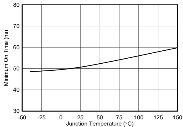
图 7-20. Minimum On Time (HO) vs. Temperature
