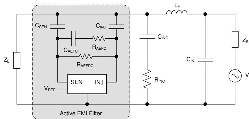
图 8-2. Active EMI Filter
