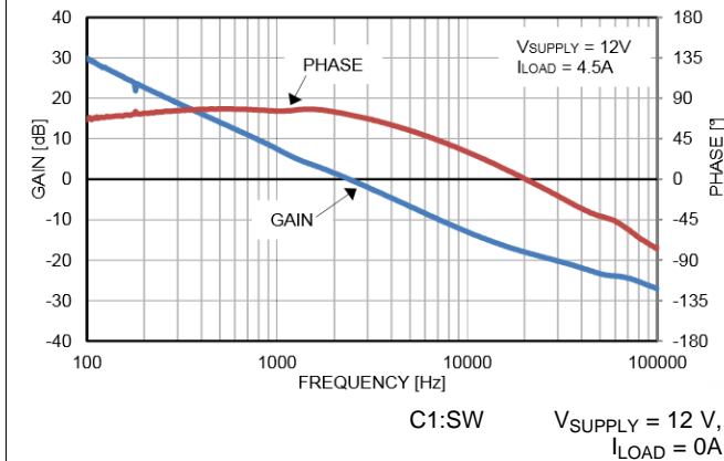
Figure 46. Loop Response
