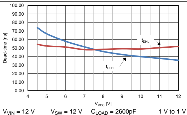
Figure 3. Dead Time vs V_{CC}
