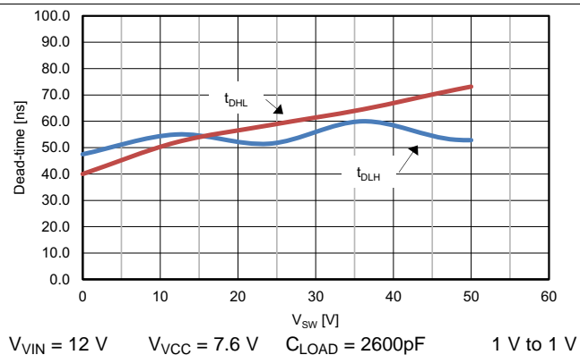
Figure 5. Dead Time vs V_{SW}
