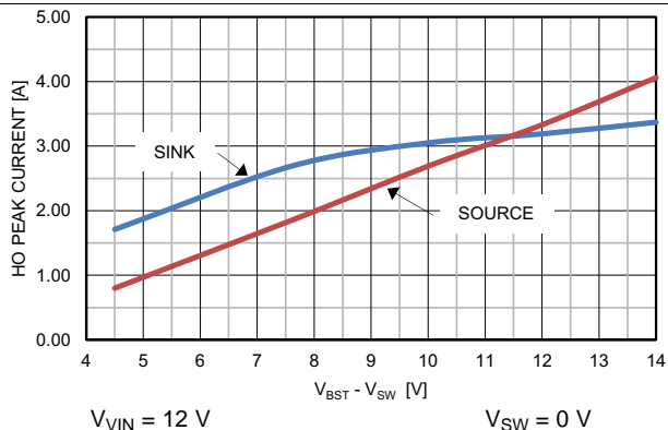
Figure 1. HO Peak Current vs V_{BST} - V_{SW}
