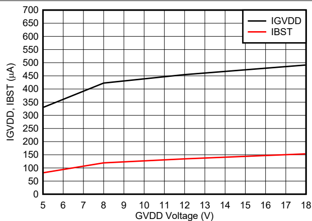
图 6-6. Quiescent Currents vs Supply Voltage
