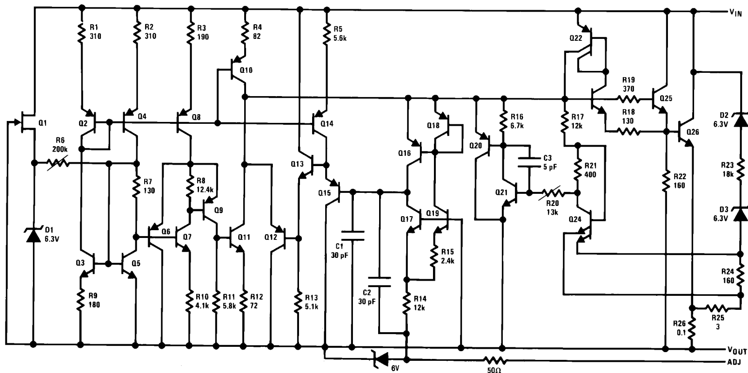
图 8-2. Simplified Device Schematic
