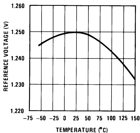
图 7-5. Temperature Stability
