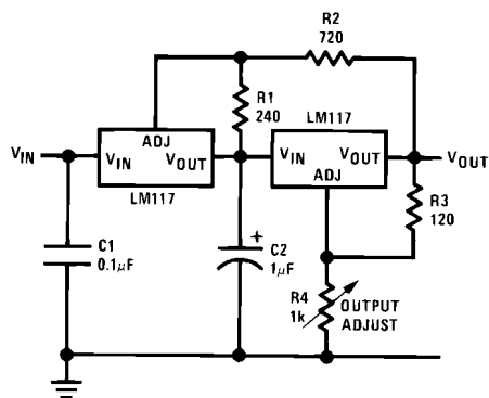
图 9-15. Tracking Preregulator
