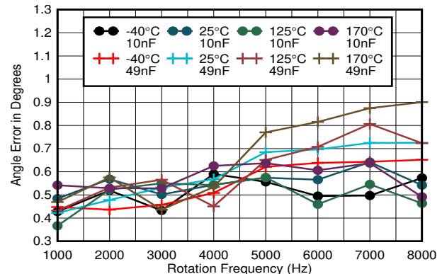
图 7-2. Angle Error VCC = 5 V, C_{OUT} < 50 \text{ nF}
