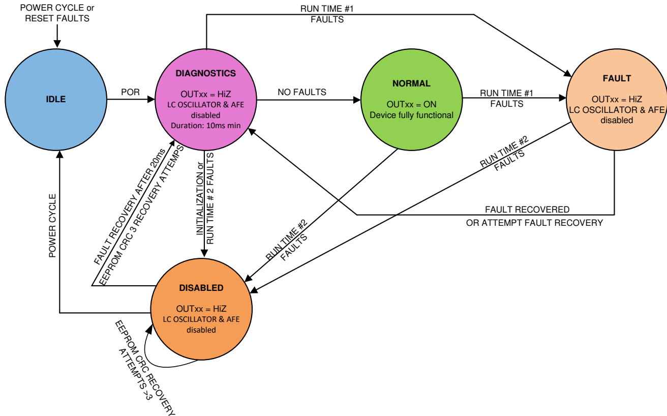
图 8-5. Device State Diagram
