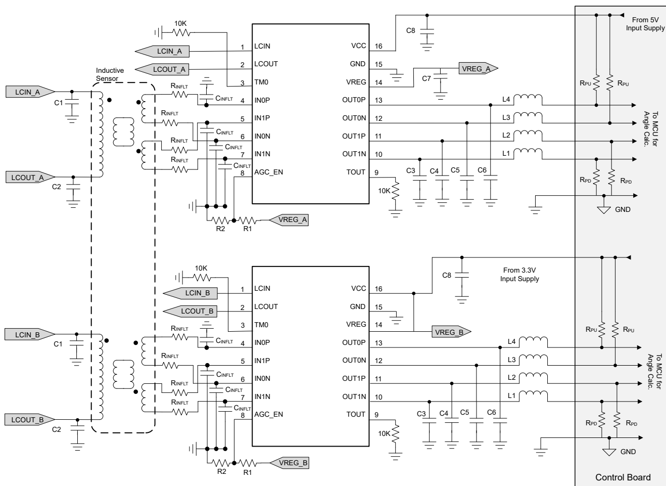
图 9-4. Application Schematic - Redundancy Mode
