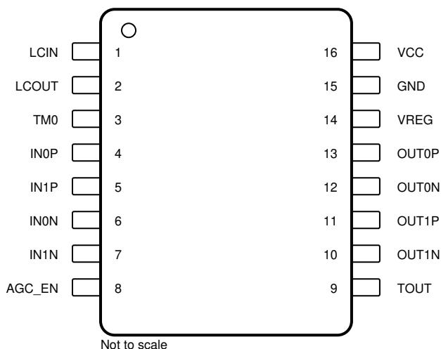
图 6-1. PW Package 16-Pin TSSOP Top View
