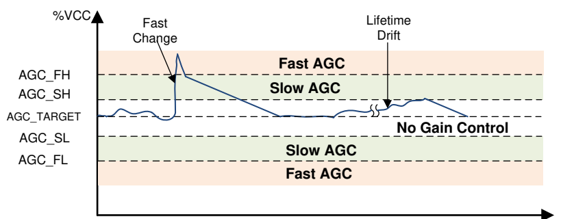
图 8-3. AGC Regulation Bands
