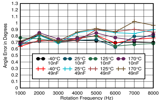
图 7-1. Angle Error VCC = 5 V, C_{OUT} < 50 \text{ nF}
