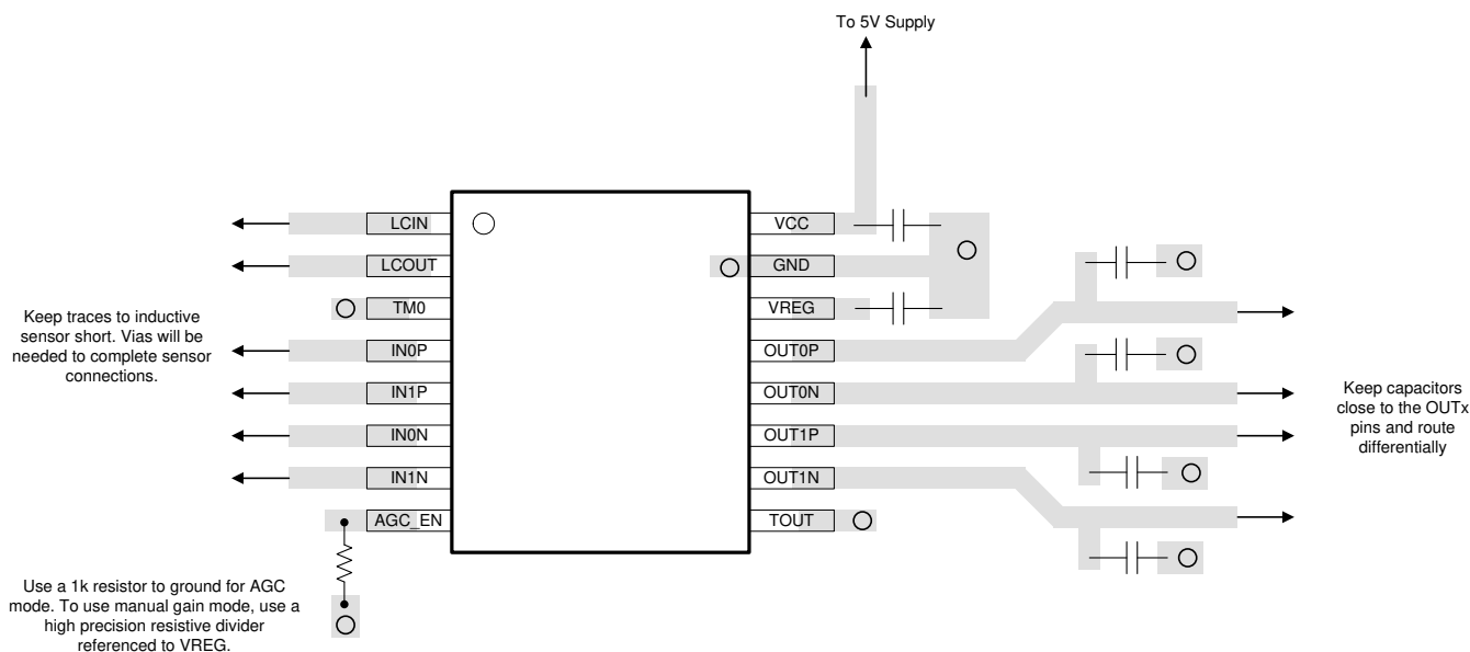
图 11-1. Layout Recommendation for the LDC5072-Q1
