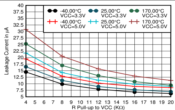
图 7-6. OUTx Pin Leakage Current When Device is in a SAFE State and Output Pulled to VCC With R Pull-up
