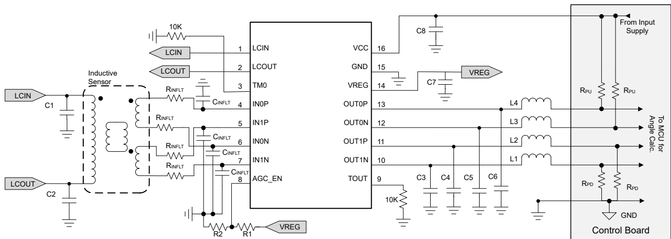
图 9-1. Application Schematic - 5-V Supply Mode
