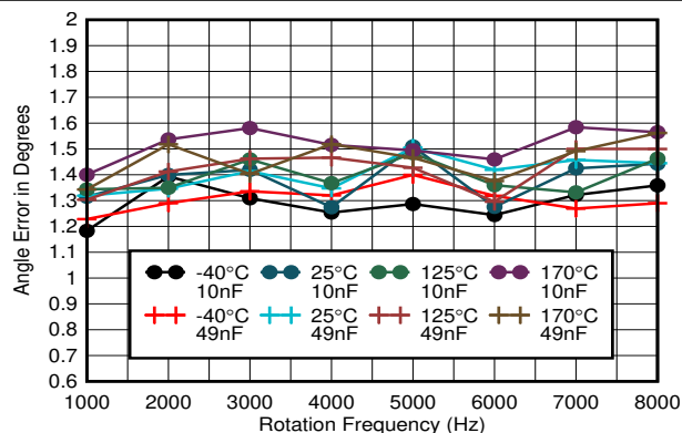
图 7-1. Angle Error VCC = 5 V, C_{OUT} < 50 \text{ nF}
