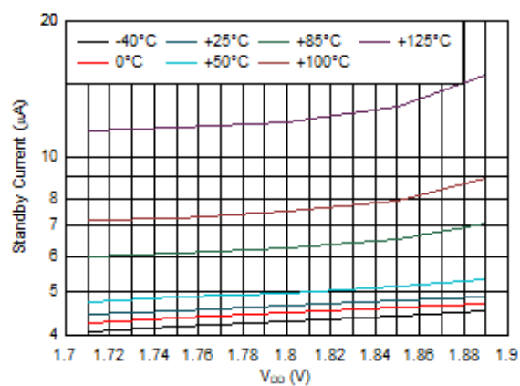
图 6-8. Standby Current vs V_{DD}
