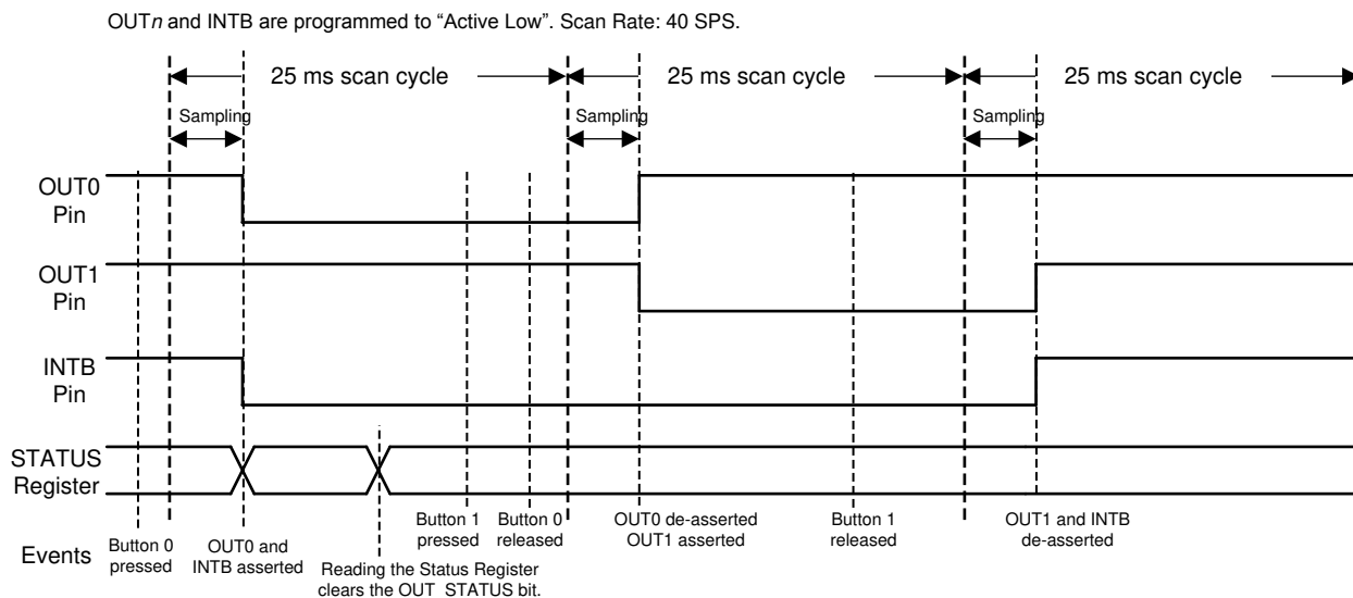
图 8-14. Timing Diagram of Multiple Button Presses
