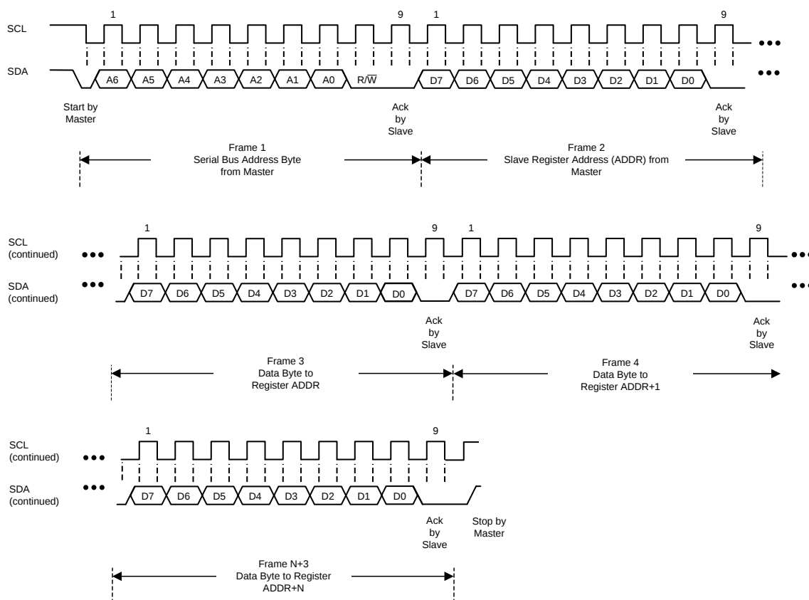
图 14. I 2 C Sequence of Writing Consecutive Registers
