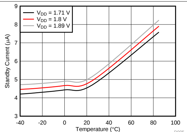
图 7. Standby Current vs Temperature
