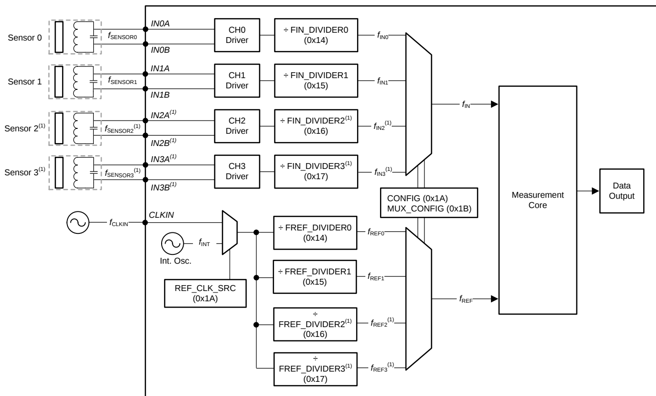
Figure 54. Clocking Diagram
