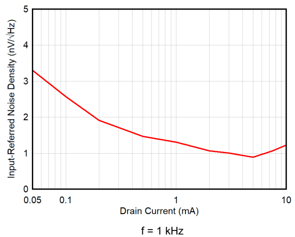
图 6-16. Input-Referred Noise Spectral Density vs Drain-to-Source Current
