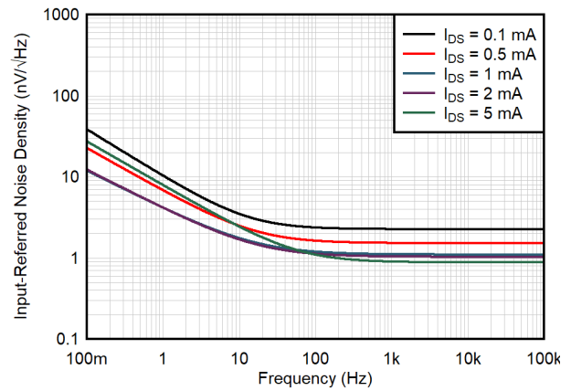
图 6-14. Input-Referred Noise Density vs Frequency
