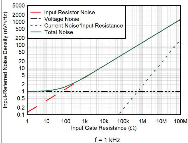
图 6-15. Noise Density Contributors vs Input Gate Resistance
