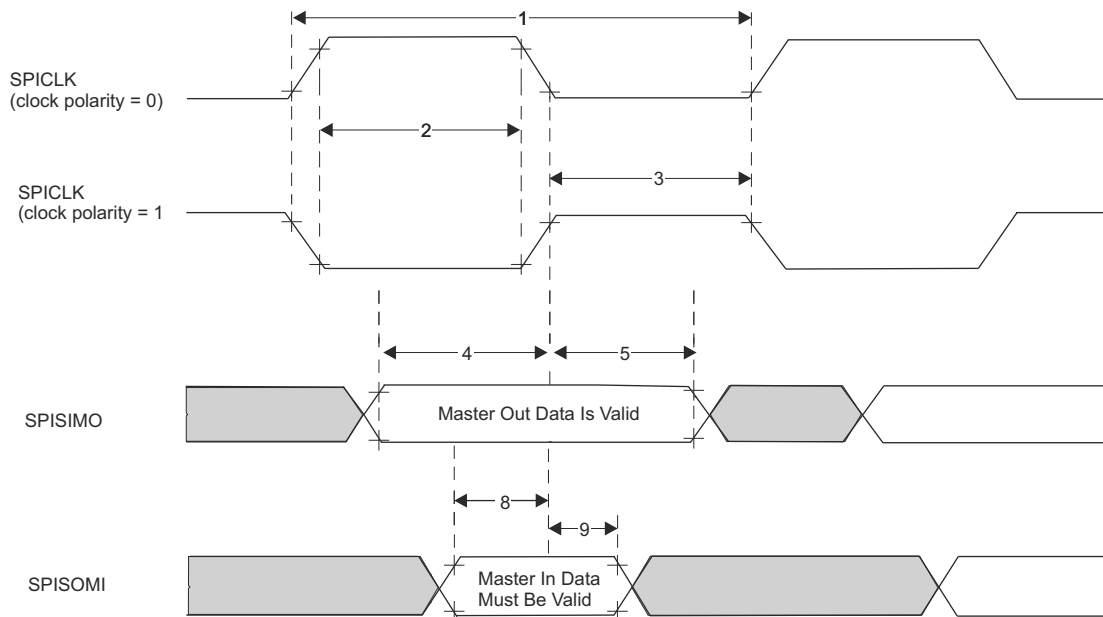
图 8-4. SPI Master Mode External Timing (CLOCK PHASE = 0)
