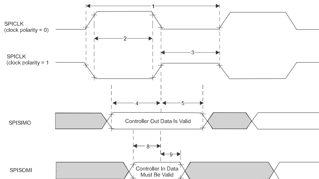
图 7-8. SPI Controller Mode External Timing (CLOCK PHASE = 0)
