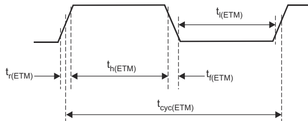
图 7-20. ETMTRACECLKOUT Timing
