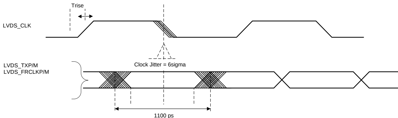
Figure 5-13. Timing Parameters
