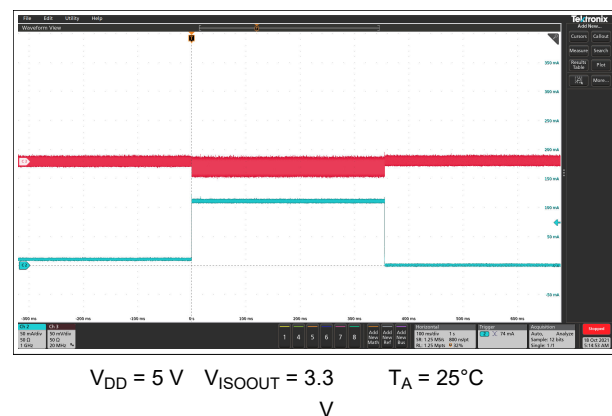
图 7-25. 10-mA to 110-mA Load Transient Response
