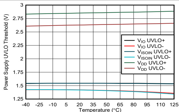
图 7-21. Power-Supply Undervoltage Threshold vs Free Air Temperature
