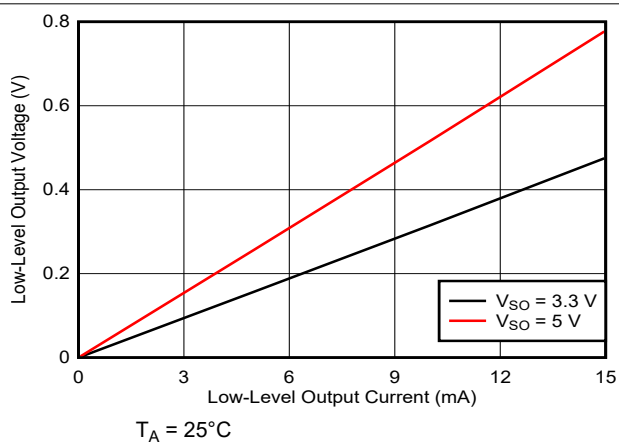
图 7-24. Low-Level Output Voltage vs Low-Level Output Current
