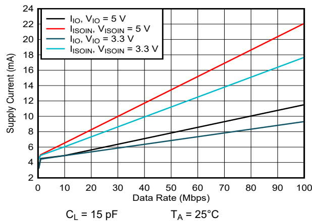
图 7-13. ISOW7741 Channel Supply Currents vs Data Rate For C_L = 15\text{ pF}
