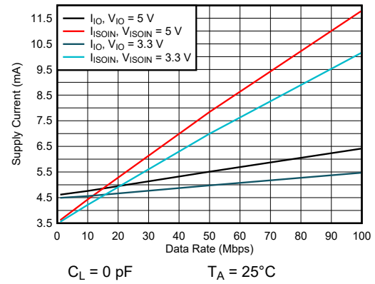
图 7-12. ISOW7740 Channel Supply Currents vs Data Rate For C_L = 0\text{ pF}
