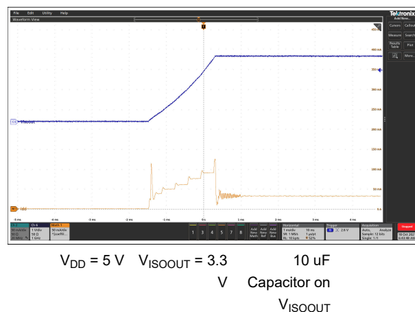
图 7-26. Soft Start at 10-mA Load For V_{ISOOUT} = 3.3 V
