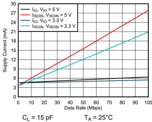
图 7-11. ISOW7740 Channel Supply Currents vs Data Rate For C_L = 15\text{ pF}
