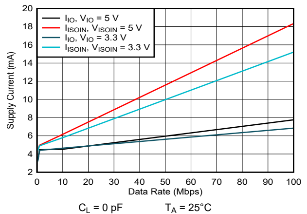
图 7-14. ISOW7741 Channel Supply Currents vs Data Rate For C_L = 0\text{ pF}
