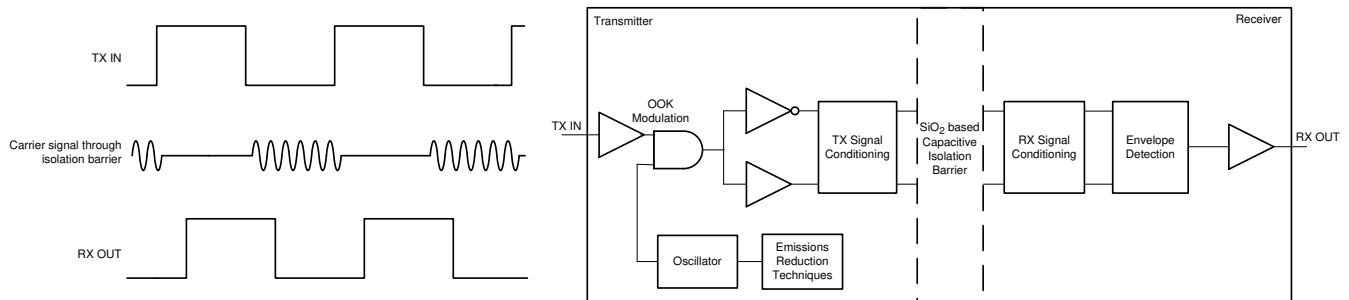
图 10-2. Signal Isolation channel
