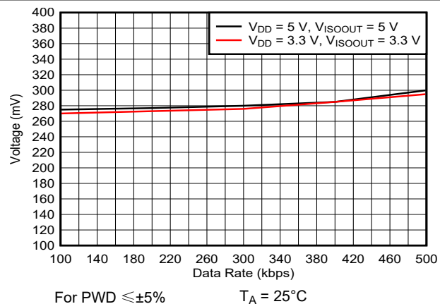
图 8-21. ISOW1412 Receiver VID vs. Data Rate - RS485 & Profibus Mode
