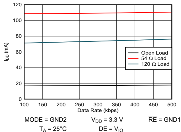
图 8-3. ISOW1412 V_{DD} Supply Current vs. Data Rate - RS485 Mode
