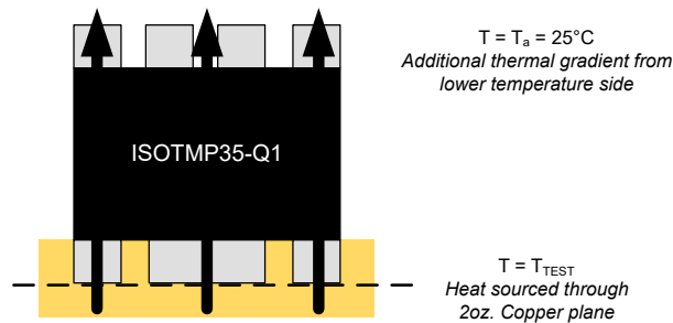
图 6-4. Directional Thermal Response Test
