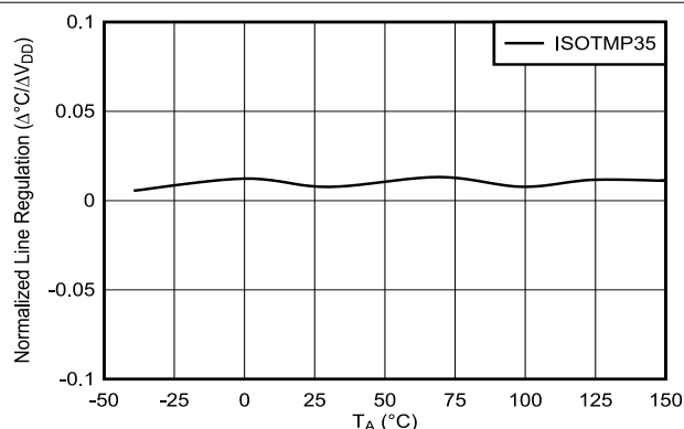
图 5-6. Line Regulation ( \Delta^\circ\text{C} / \Delta V_{DD} ) vs Ambient Temperature
