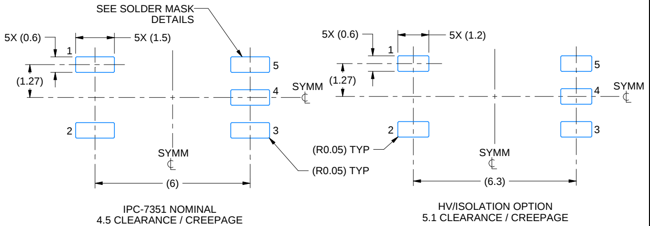
LAND PATTERN EXAMPLE EXPOSED METAL SHOWN SCALE: 7X
