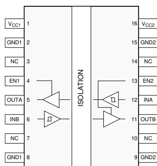
图 4-2. DWW Package 16-Pin (SOIC) Top View
