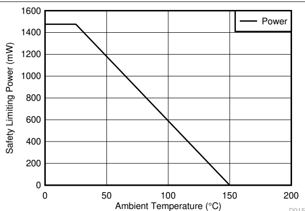
图 5-2. Thermal Derating Curve for Safety Limiting Power per VDE
