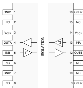
图 4-1. DW Package 16-Pin (SOIC) Top View
