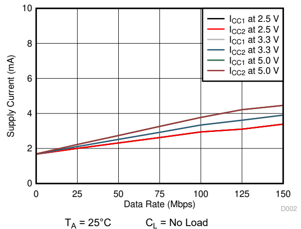
图 5-4. Supply Current vs Data Rate (With No Load)
