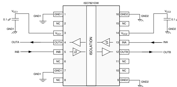
图 8-2. Typical ISO7821 Circuit Hook-up
