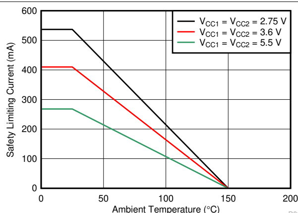
图 5-1. Thermal Derating Curve for Safety Limiting Current per VDE
