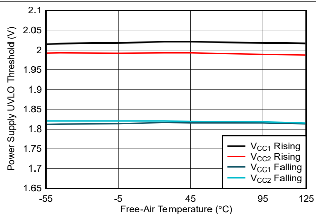
图 5-11. Power Supply Undervoltage Threshold vs Free-Air Temperature
