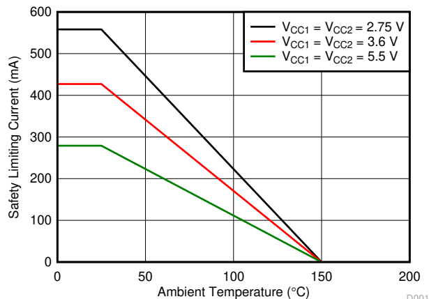
图 5-1. Thermal Derating Curve for Safety Limiting Current per VDE for DW-16 Package
