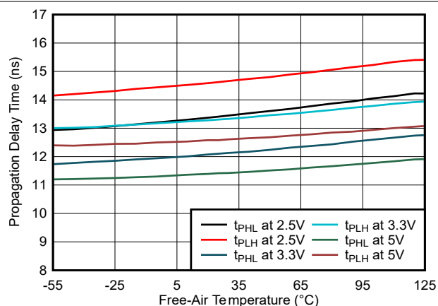
图 5-12. Propagation Delay Time vs Free-Air Temperature
