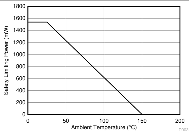
图 5-3. Thermal Derating Curve for Safety Limiting Power per VDE for DW-16 Package
