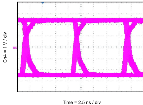
图 8-4. Eye Diagram at 100 Mbps PRBS 2 16 - 1, 5 V and 25°C
