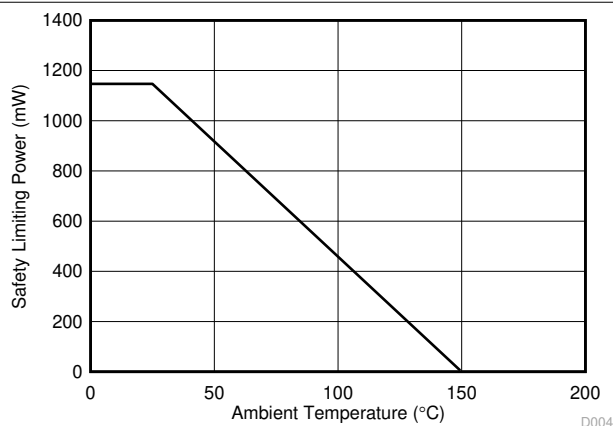
图 5-4. Thermal Derating Curve for Safety Limiting Power per VDE for DBQ-16 Package
