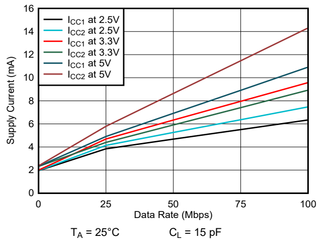
图 5-7. ISO7731-Q1 Supply Current vs Data Rate (With 15-pF Load)
