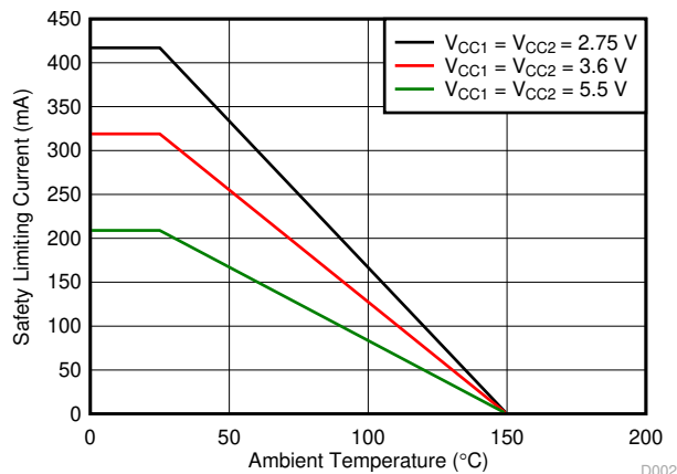
图 5-2. Thermal Derating Curve for Safety Limiting Current per VDE for DBQ-16 Package
