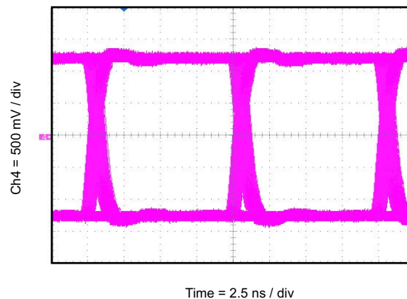
图 8-6. Eye Diagram at 100 Mbps PRBS 2 16 - 1, 2.5 V and 25°C
