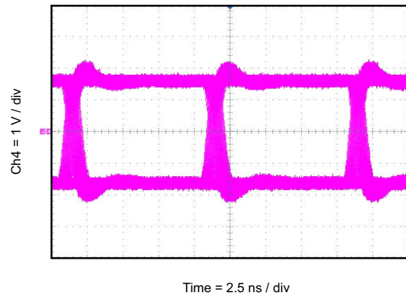
图 8-5. Eye Diagram at 100 Mbps PRBS 2 16 - 1, 3.3 V and 25°C
