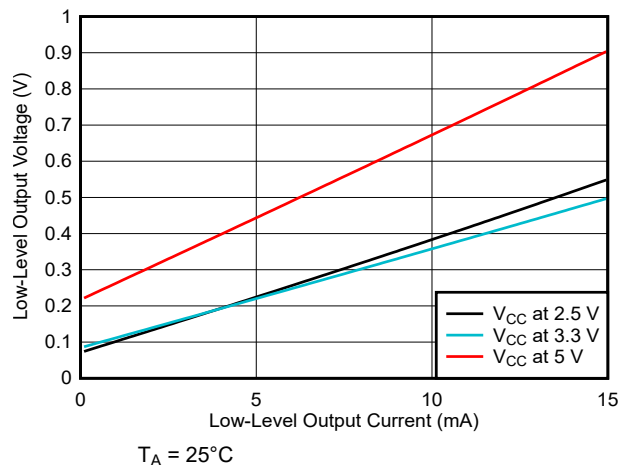
图 5-10. Low-Level Output Voltage vs Low-Level Output Current
