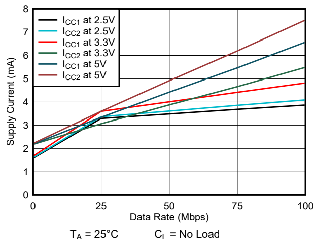
图 5-6. ISO7730 Supply Current vs Data Rate (With No Load)
