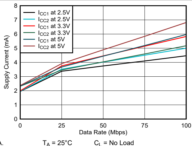
图 5-8. ISO7731 Supply Current vs Data Rate (With No Load)
