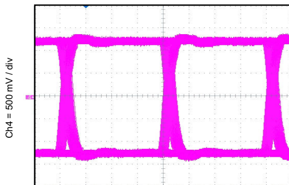
图 8-4. Eye Diagram at 100 Mbps PRBS 2 16 - 1, 5 V and 25°C
