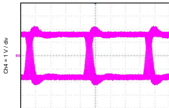
图 8-5. Eye Diagram at 100 Mbps PRBS 2 16 - 1, 3.3 V and 25°C
