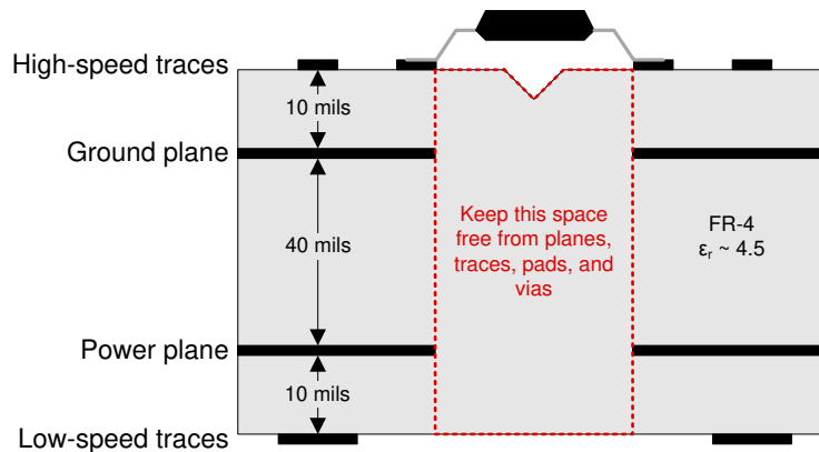
图 8-5. Recommended Layer Stack
