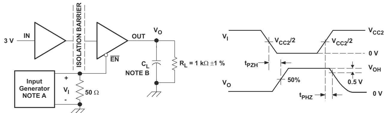
图 7-2. ISO722 Sleep-Mode High-Level Output Test Circuit and Voltage Waveforms
