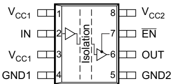
图 5-2. ISO722 and ISO722M D Package 8-Pin SOIC Top View
