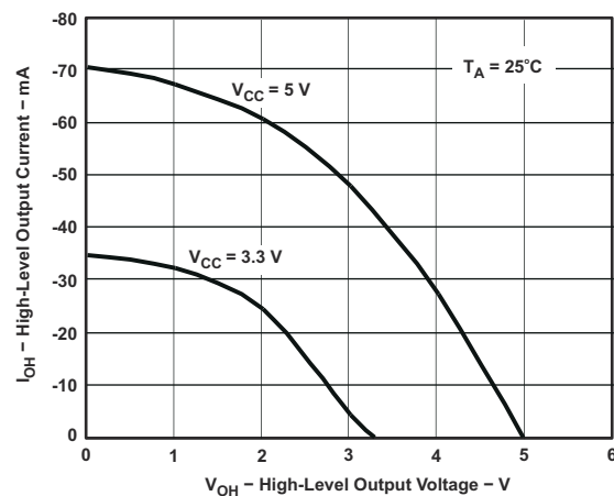
图 6-8. High-Level Output Current vs High-Level Output Voltage
