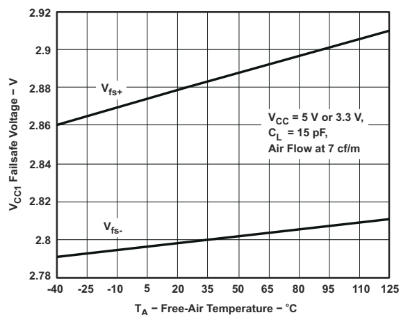
图 6-7. V CC1 Failsafe Threshold Voltage vs Free-Air Temperature
