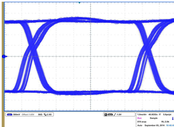
图 9-5. ISO721M Eye Diagram at 150 Mbps, 3.3 V, and 25°C
