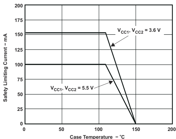
图 9-6. Thermal Derating Curve for Limiting Current per VDE
