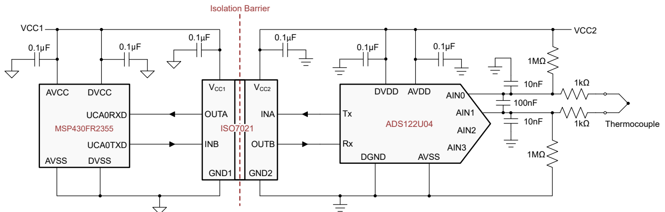
图 9-3. Isolated UART for a Temperature Field Transmitter
